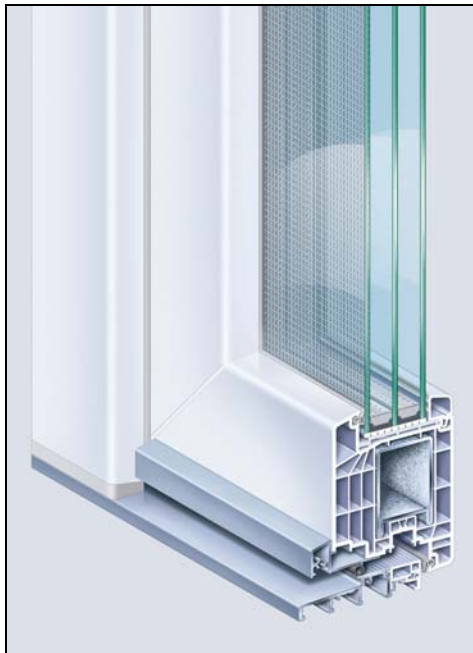
The new "Kömmerling 88plus" residential door system with inward opening sash.
