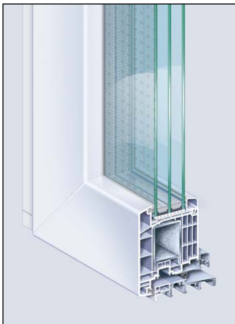
The new "Kömmerling 88plus" residential door system with outward opening sash
