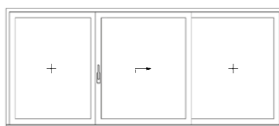
One lift/sliding sash and two fixed panes
