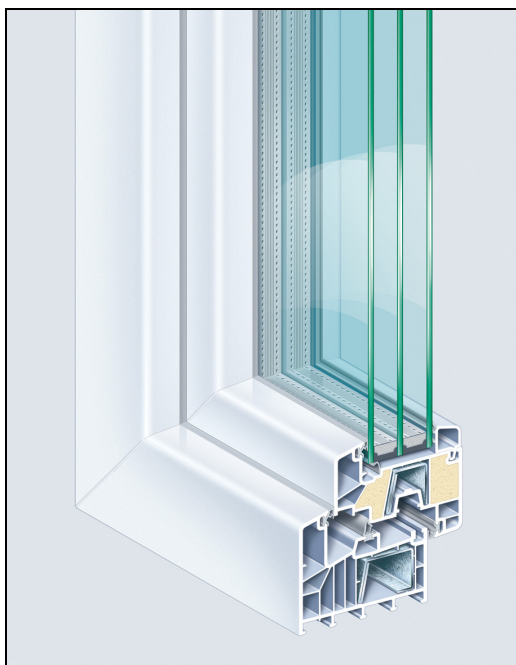
proEnergyTec – This example on the Kömmerling 88plus system fulfils the passive house standard set out in the ift-guideline WA-15/2.
